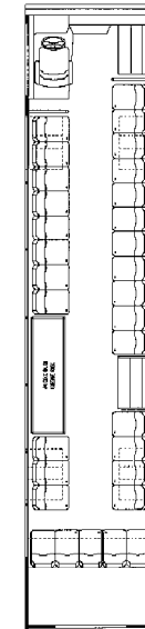
MODEL CT-380 31-Passenger Perimeter Seating
